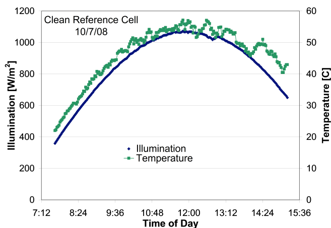
Fig. 1. Example of readable plot using different colors and line styles for clarity.
